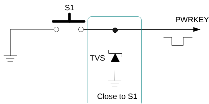
Figure 12: Turn on the Module Using a Button
