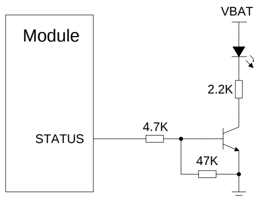
Figure 28: Reference Circuits of STATUS
