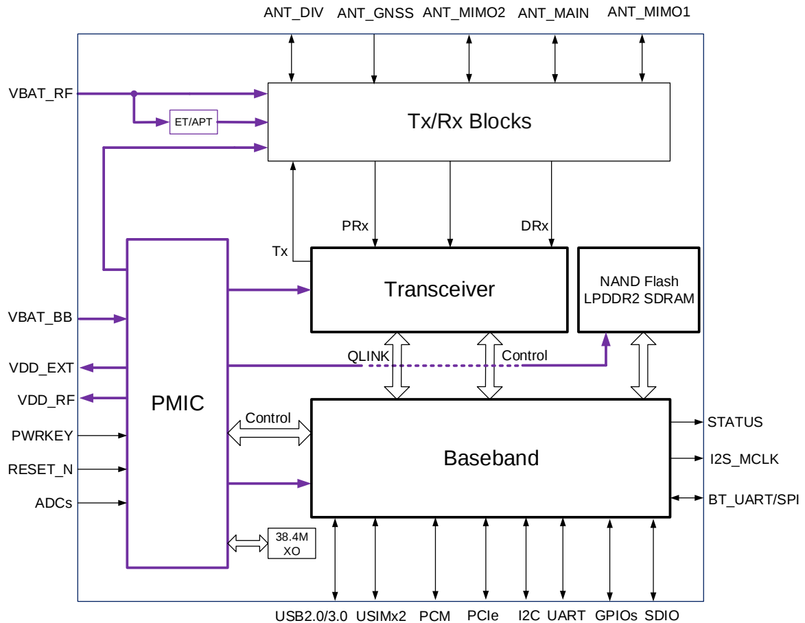
Figure 1: Functional Diagram
