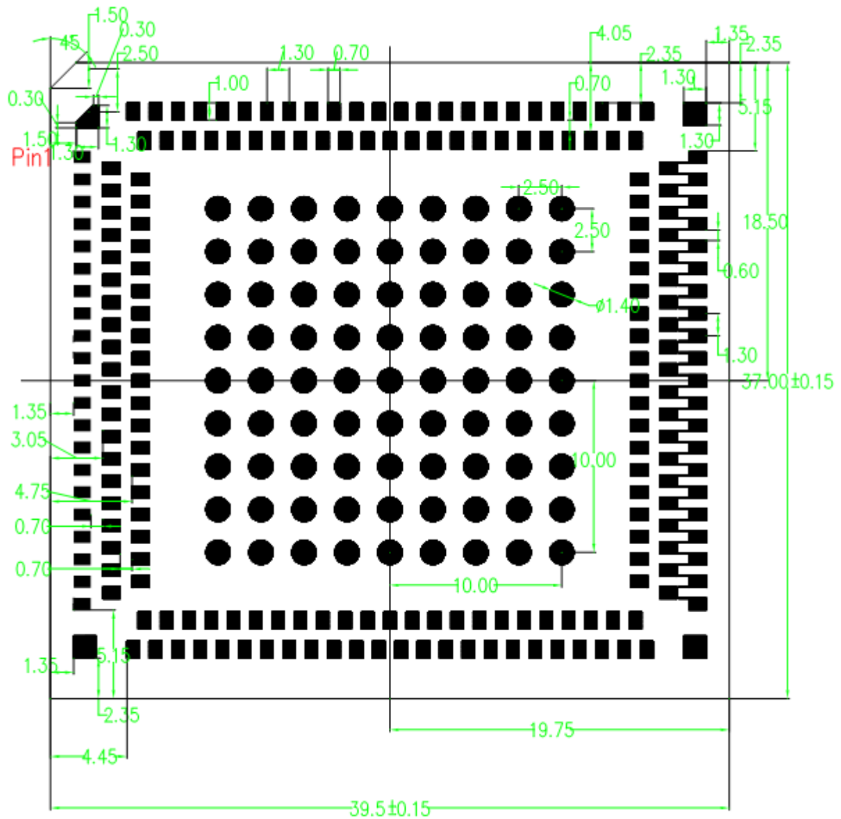
Figure 45: Module Bottom Dimensions (Top View)
