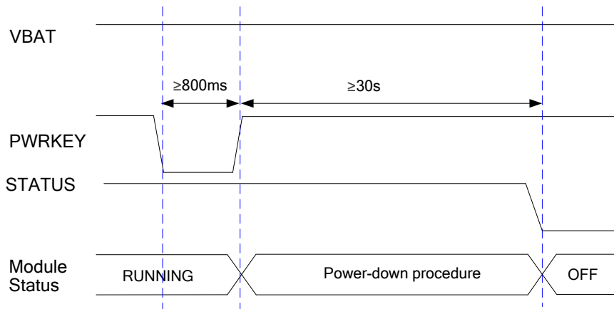
Figure 14: Timing of Turning off the Module
