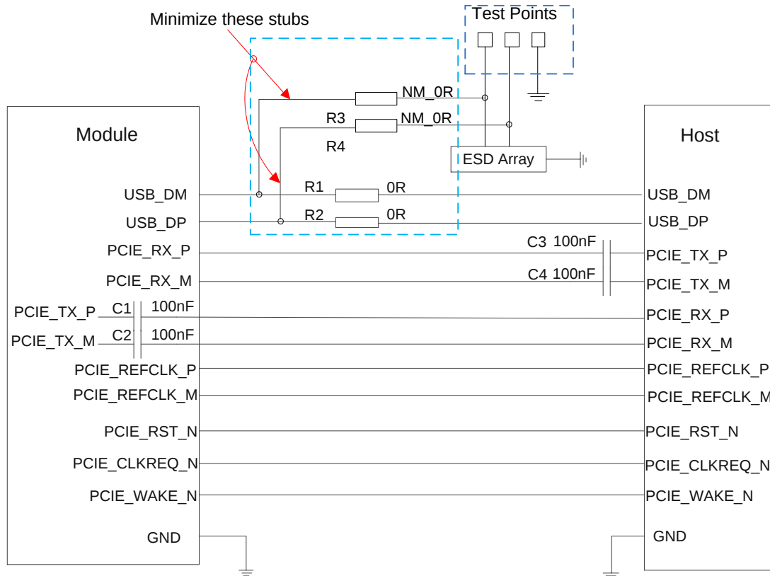
Figure 30: PCIe Interface Reference Circuit (EP Mode)
