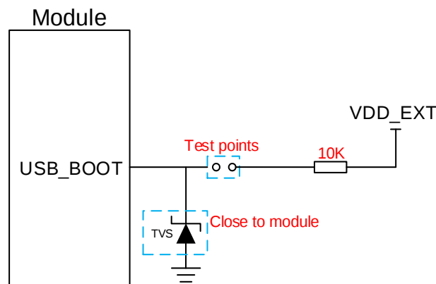
Figure 32: Reference Circuit of USB_BOOT
