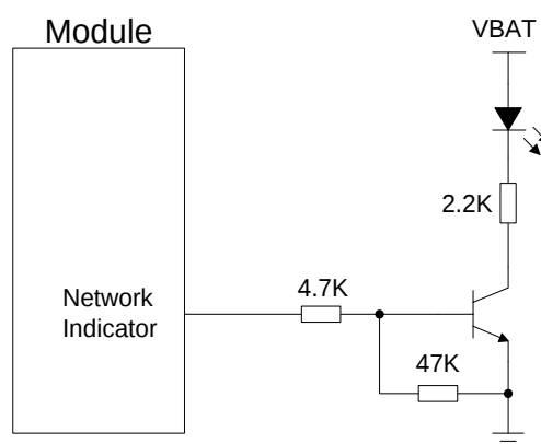
Figure 27: Reference Circuit of the Network Indicator
