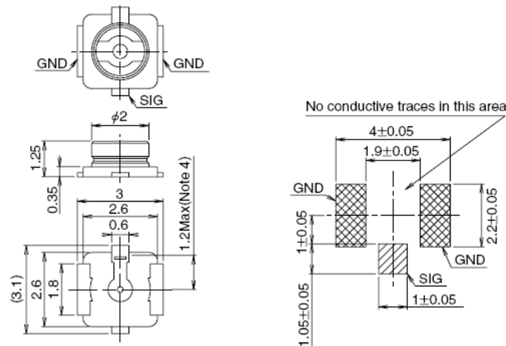
Figure 40: Dimensions of the Receptacle (Unit: mm)
