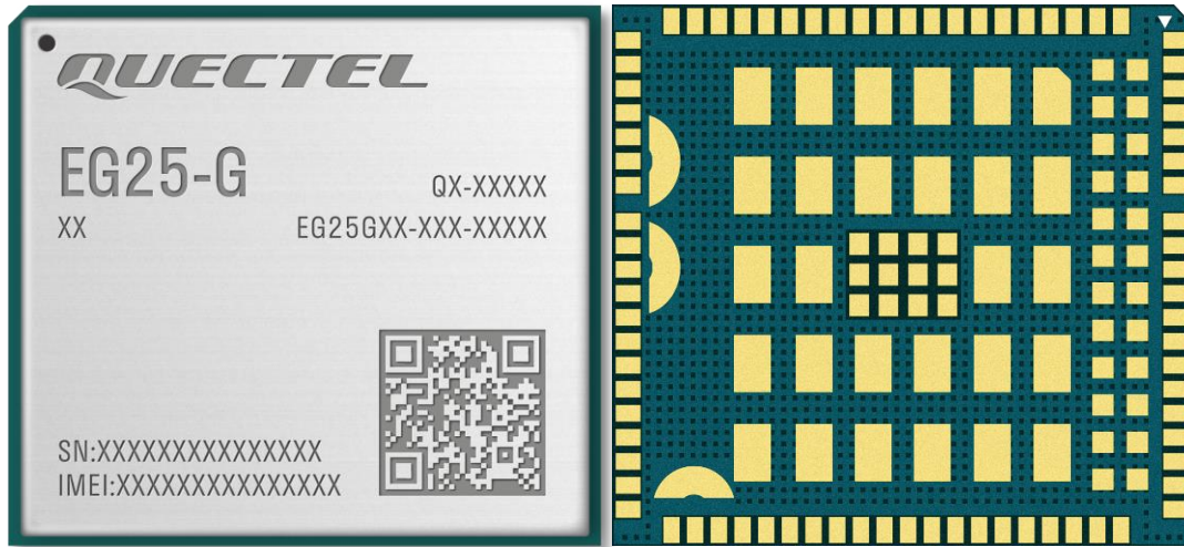
Figure 49: Top and Bottom Views of the Module
