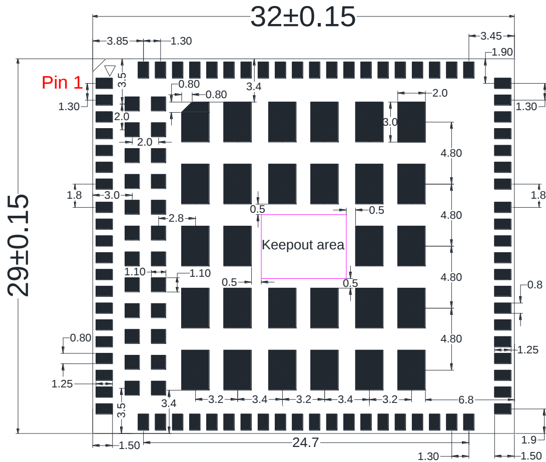
Figure 47: Recommended Footprint
