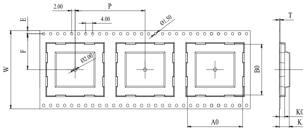
Figure 51: Carrier Tape Dimension Drawing (Unit: mm)
