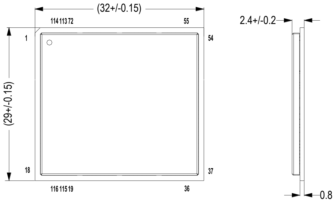
Figure 45: Module Top and Side Dimensions
