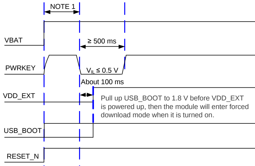
Figure 33: Timing of Entering Forced Download Mode
