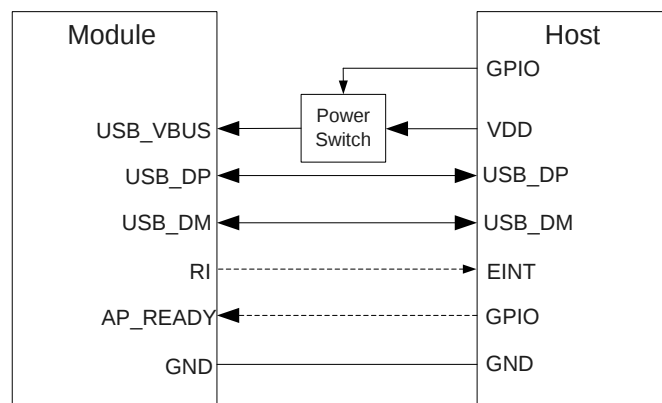
Figure 7: Sleep Mode Application Without Suspend Function
