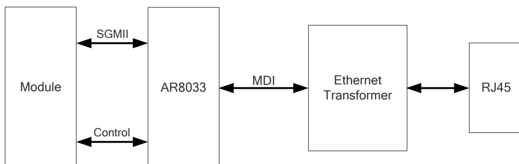
Figure 28: Simplified Block Diagram for Ethernet Application
