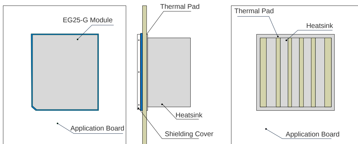
Figure 44: Referenced Heatsink Design (Heatsink at the Backside of Your PCB)
