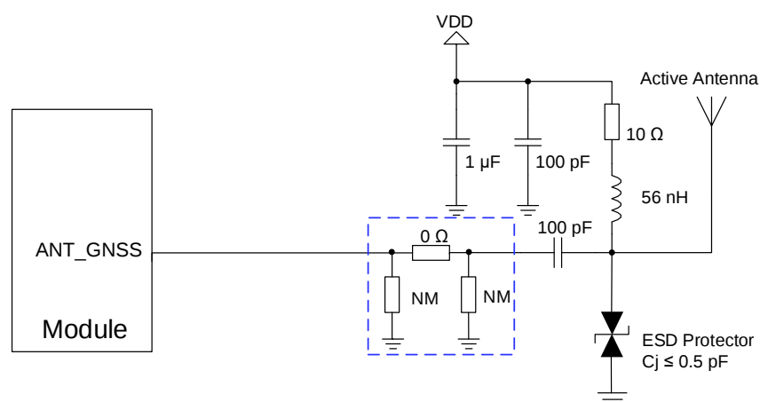
Figure 35: Reference Circuit of GNSS Antenna Interface
