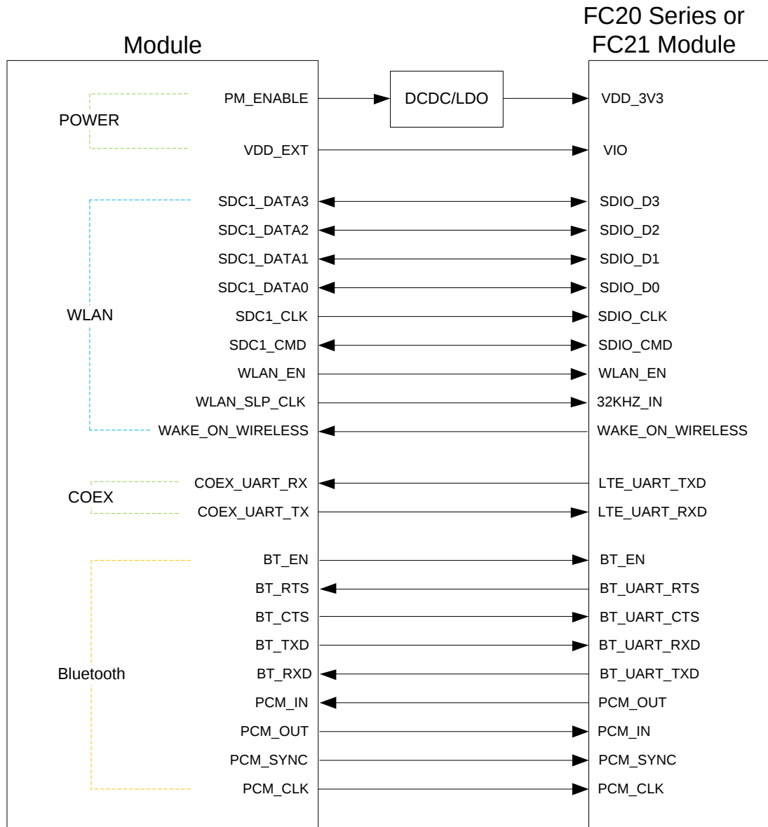
Figure 27: Reference Circuit of Wireless Connectivity Interfaces with FC20 Series or FC21 Module
