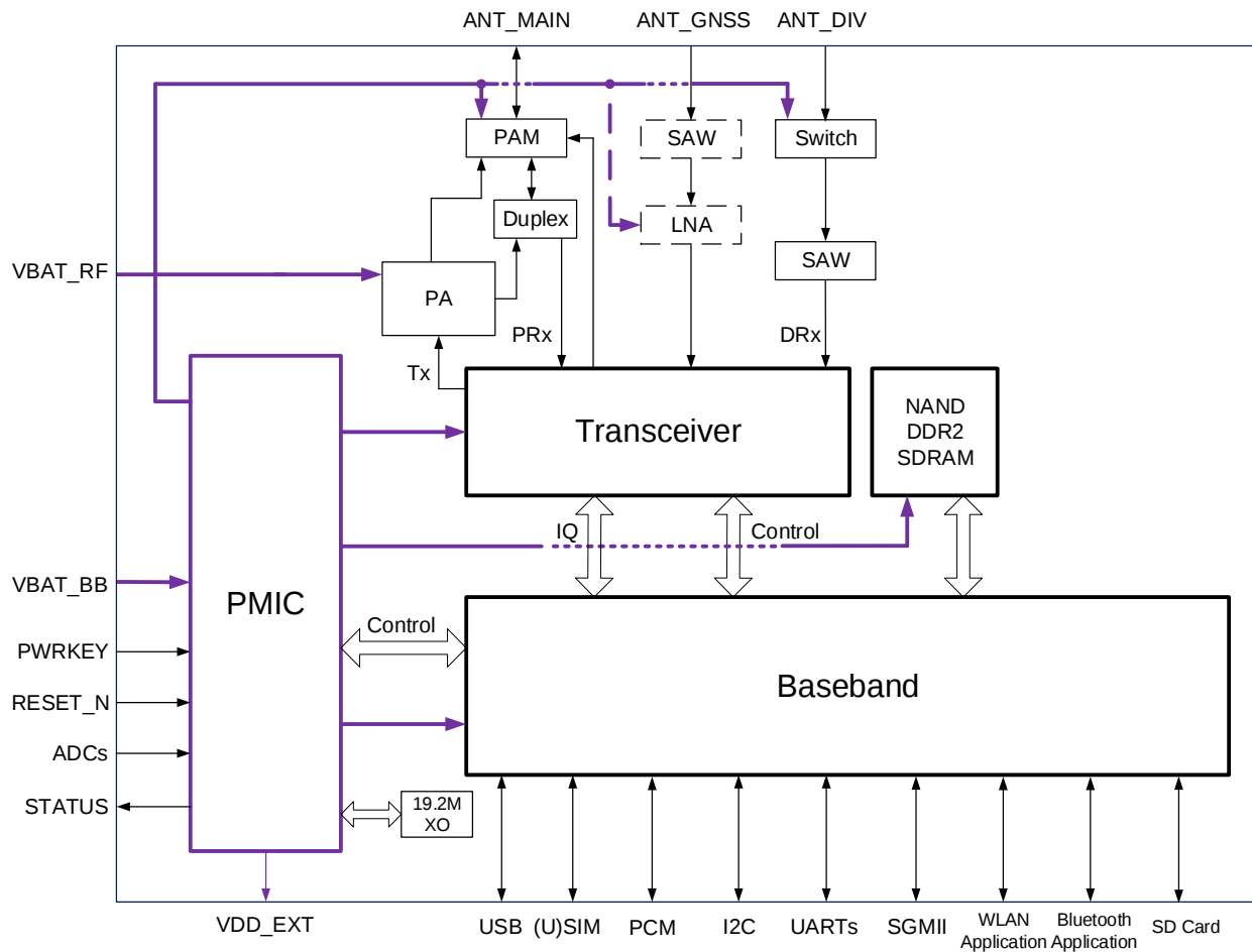
Figure 1: Functional Diagram
