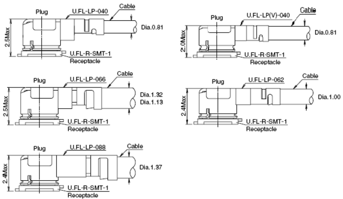
Figure 42: Space Factor of Mated Connectors (Unit: mm)
