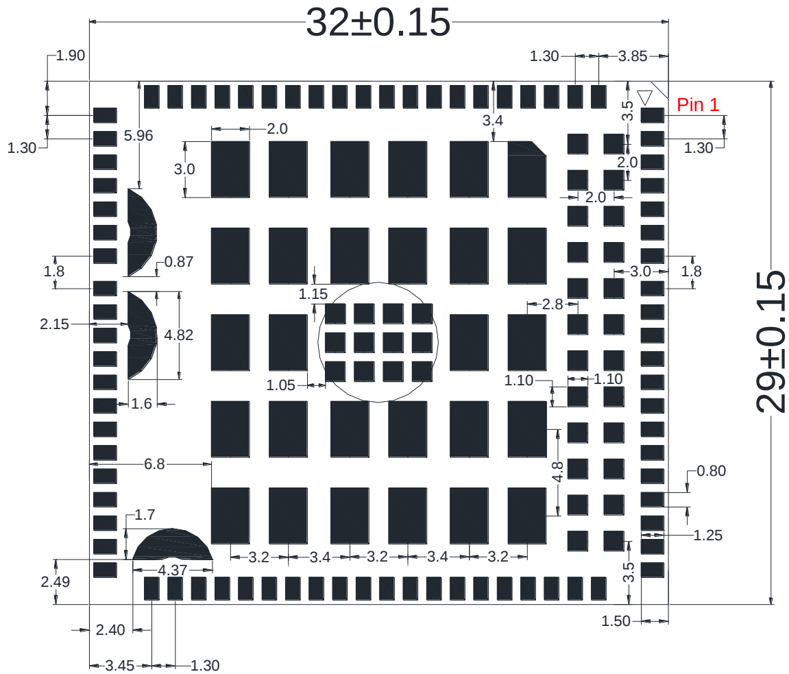
Figure 46: Module Bottom Dimensions (Bottom View)
