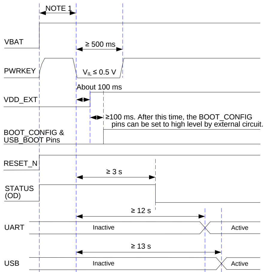
Figure 13: Power-up Timing
