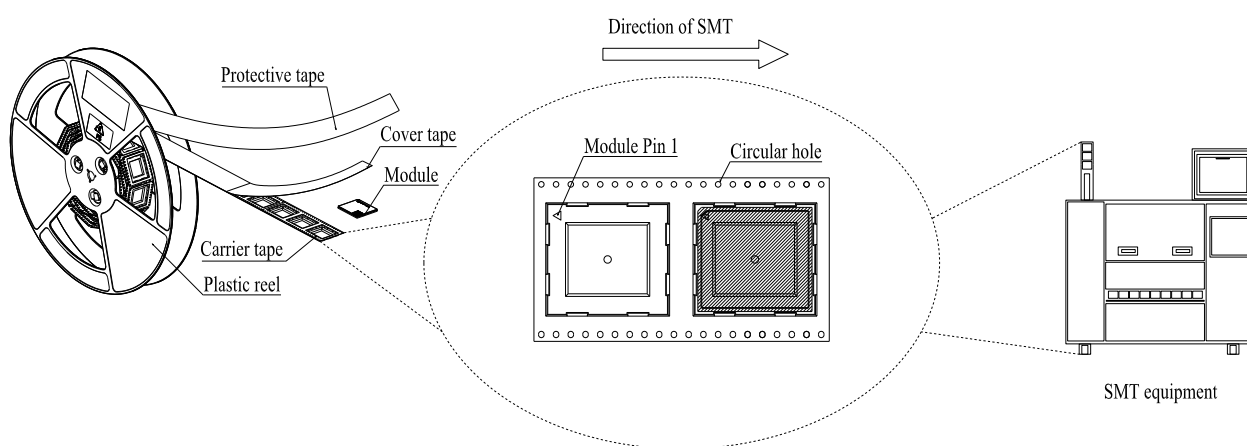
Figure 53: Mounting Direction
