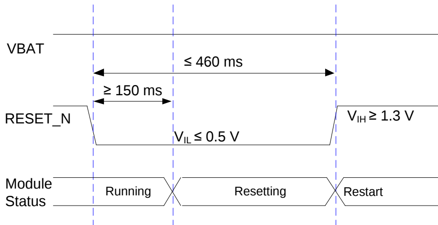
Figure 17: Timing of Resetting Module
