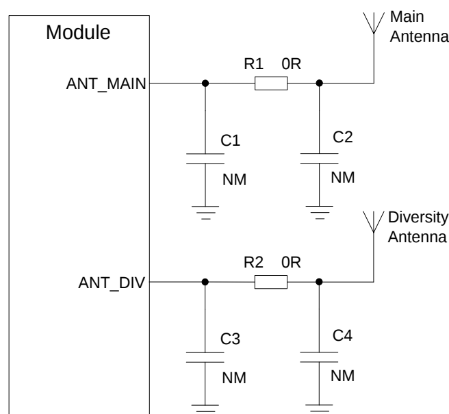
Figure 34: Reference Circuit of Cellular Antenna Interfaces
