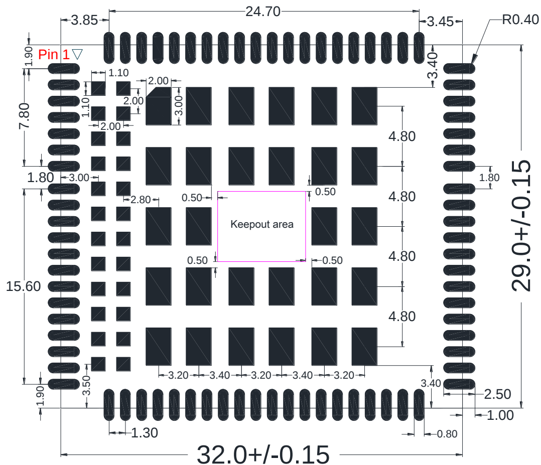
Figure 48: Recommended Compatible Footprint
